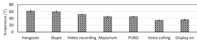
Figure 5: Mean steady-state temperatures of each scenario with three Nexus 5X phones. The error bar shows standard deviation.
