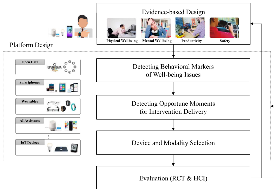
Fig. 1. Intelligent positive computing framework for delivering in-situ, intelligent, in-time, intimate, and incorporated services (i.e., the so-called “five I’s” of intelligent positive computing).
