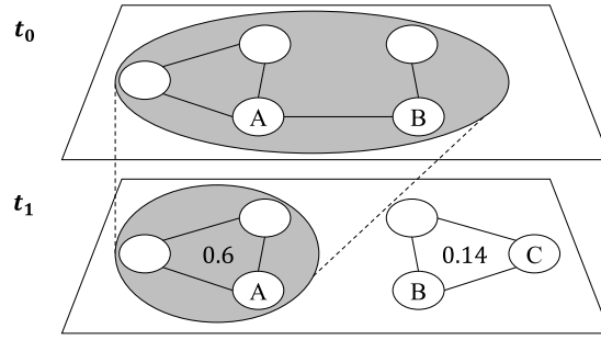
Fig. 2. Example of a group mobility trace construction from time t_0 to t_1 . The group mobility trace is represented as a combination (dotted lines) of the similar connected components (gray circles).
