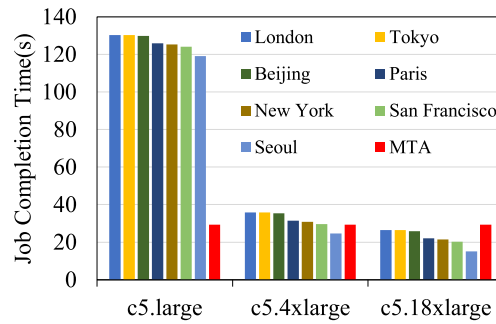
Fig. 8. Job completion time of MTA and the task offloading approach.
