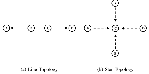
Fig. 7. Simulation Topologies
