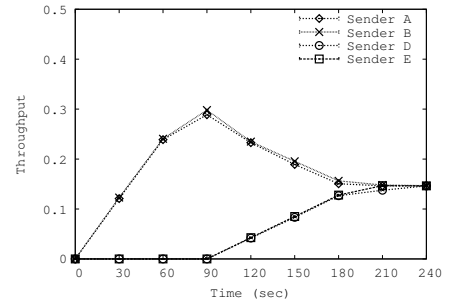
Fig. 11. 4Senders-1Sink: M-FAMA's throughput convergence under homogeneous traffic
